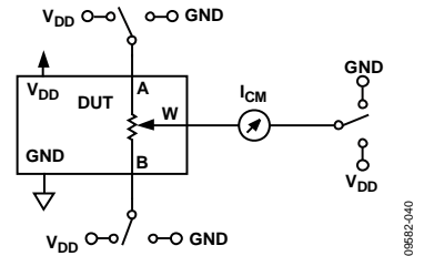
Figure 40. Common-Mode Leakage Current
