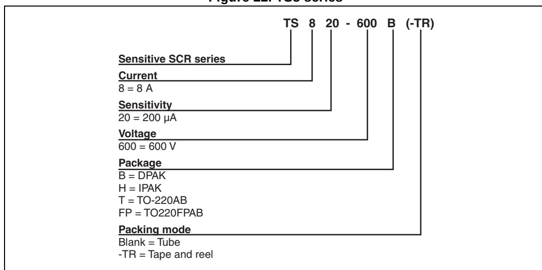
Figure 22. TS8 series
