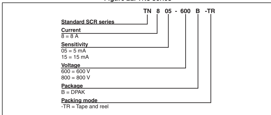
Figure 21. TN8 series
