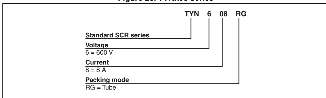
Figure 23. TYNx08 series
