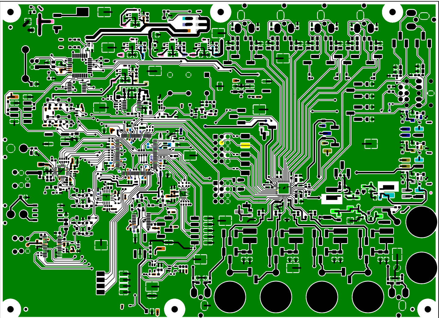
Figure 15. Top-Side Layer
