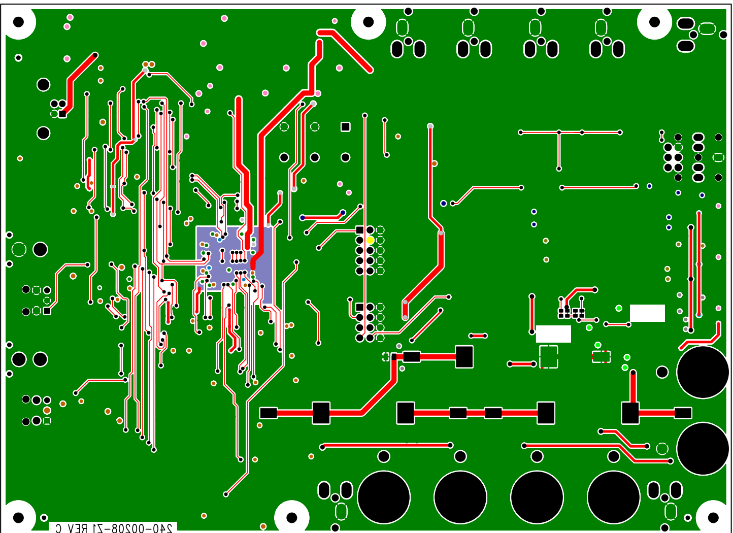
Figure 18. Bottom-Side Layer
