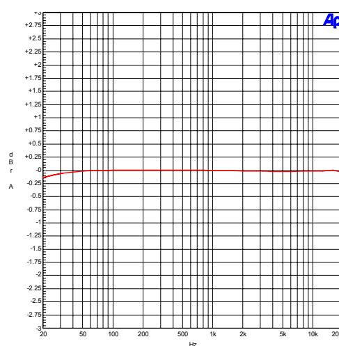
Figure 22. Freq. Resp. - S/PDIF Input to HP Output
