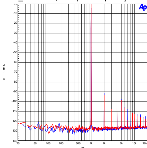
Figure 19. FFT - S/PDIF Input to HP Output @ -1 dBFS
