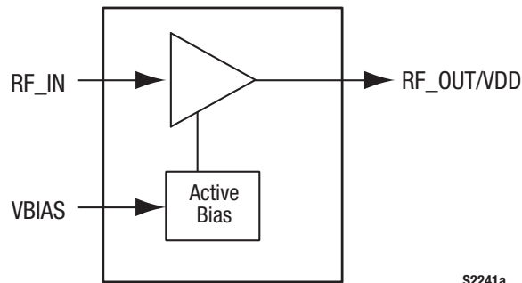
Figure 1. SKY67151-396LF Block Diagram
