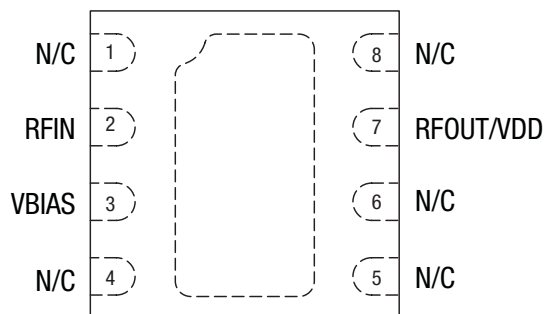
Figure 2. SKY67151-396LF Pinout – 8-Pin DFN (Top View)
