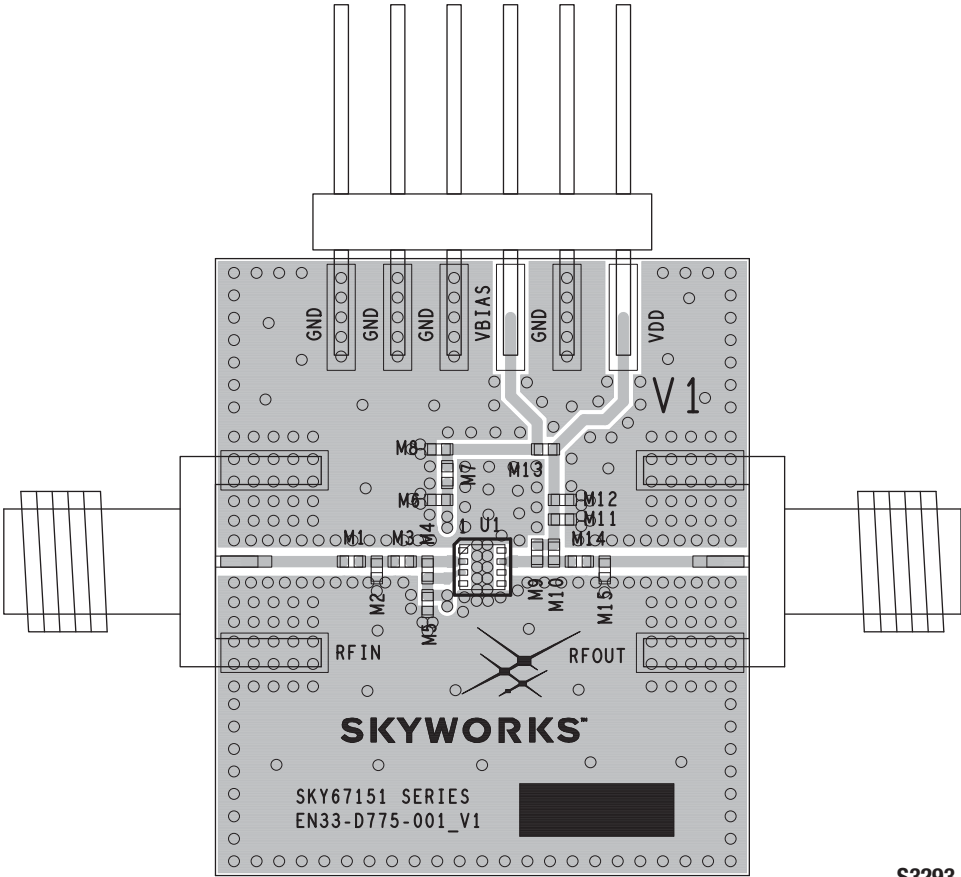
Figure 22. SKY67151-396LF Evaluation Board Assembly Diagram
