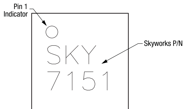
Figure 26. Typical Case Markings (Top View)
