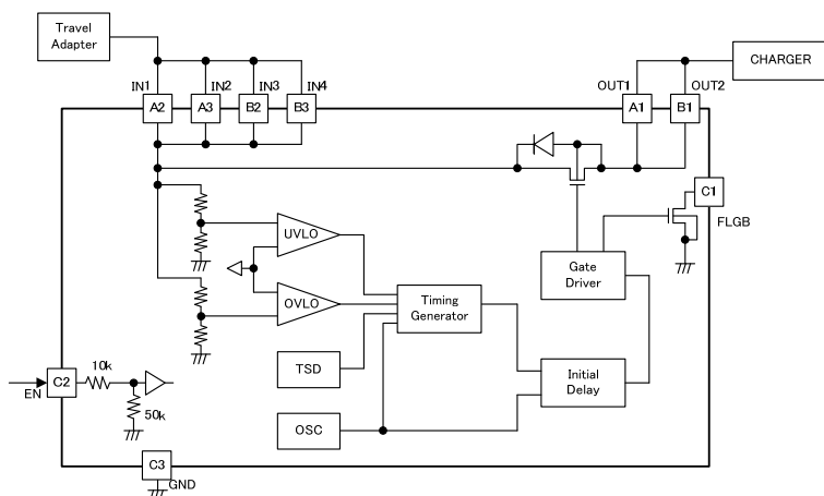
Figure1. Block Diagram
