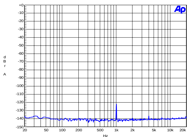
Figure 29. 192 kHz, Crosstalk
