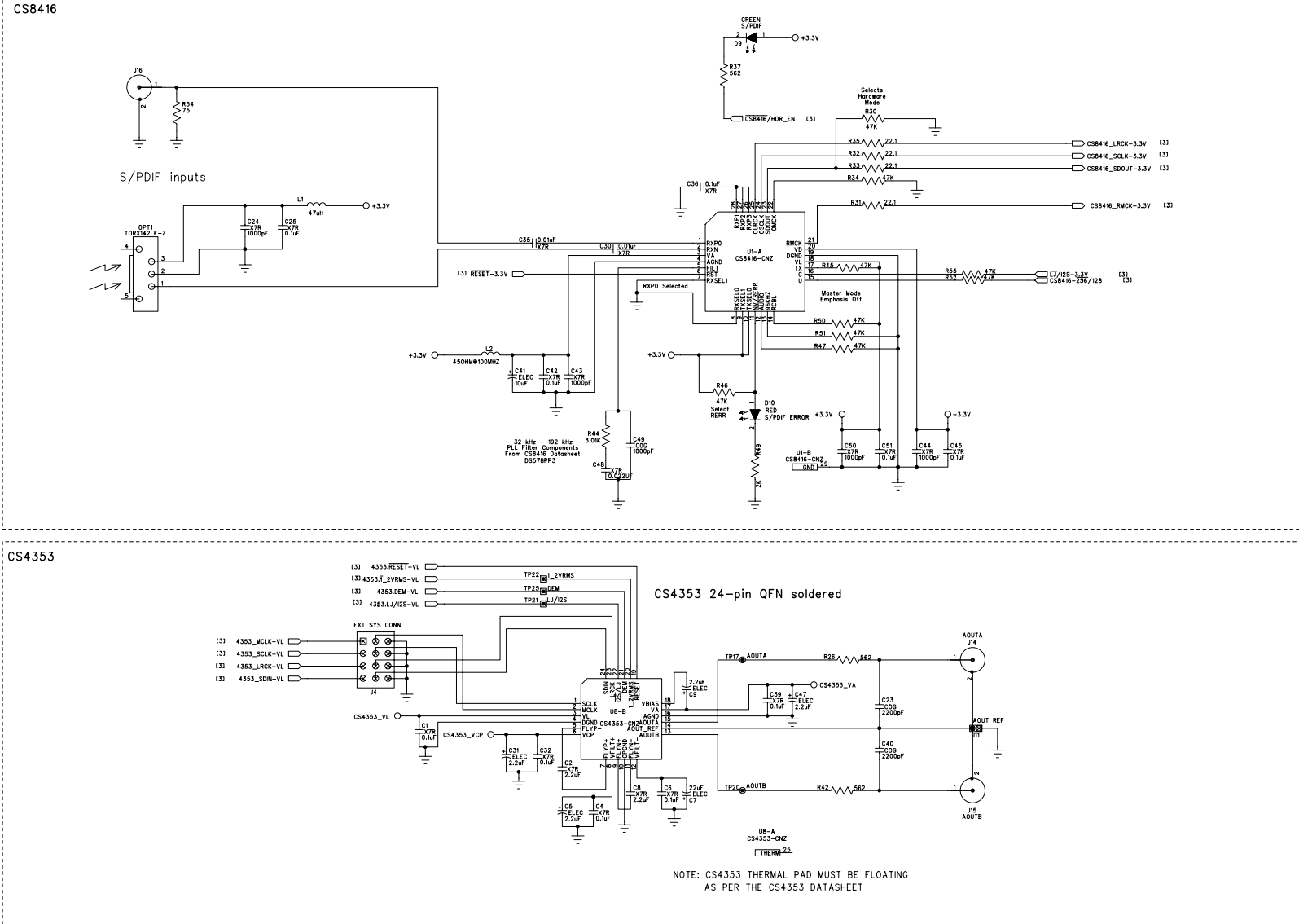
Figure 32. CS8416 and CS4353
