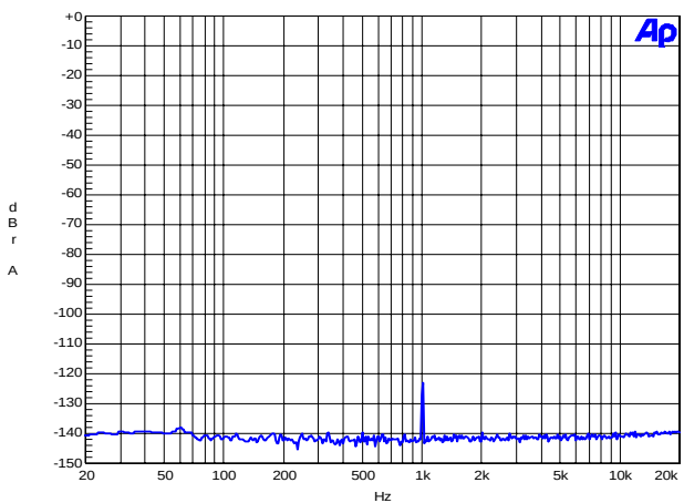
Figure 9. 48 kHz, Crosstalk
