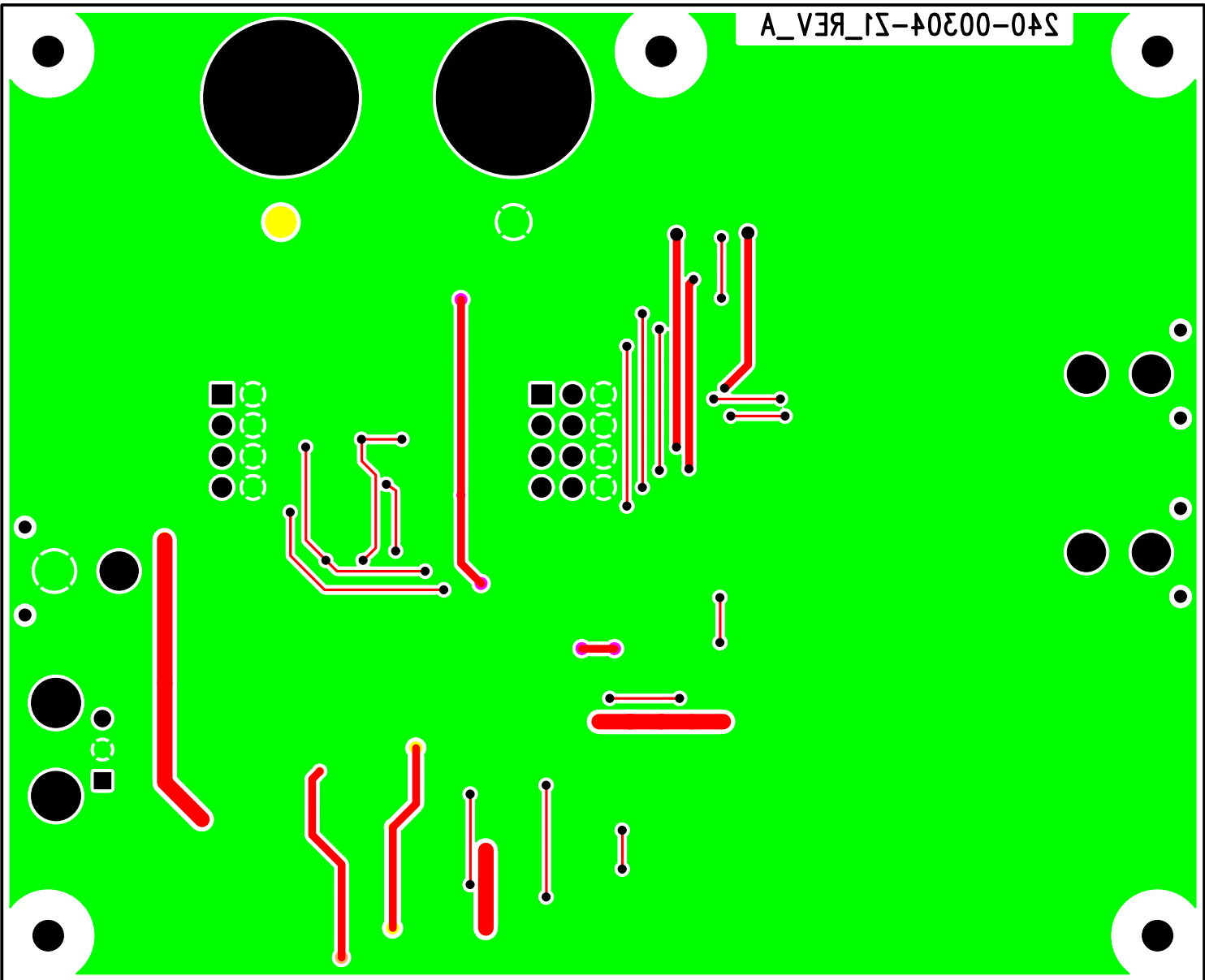
Figure 36. Bottom Side
