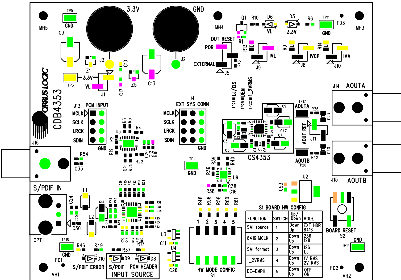
Figure 34. Silkscreen Top
