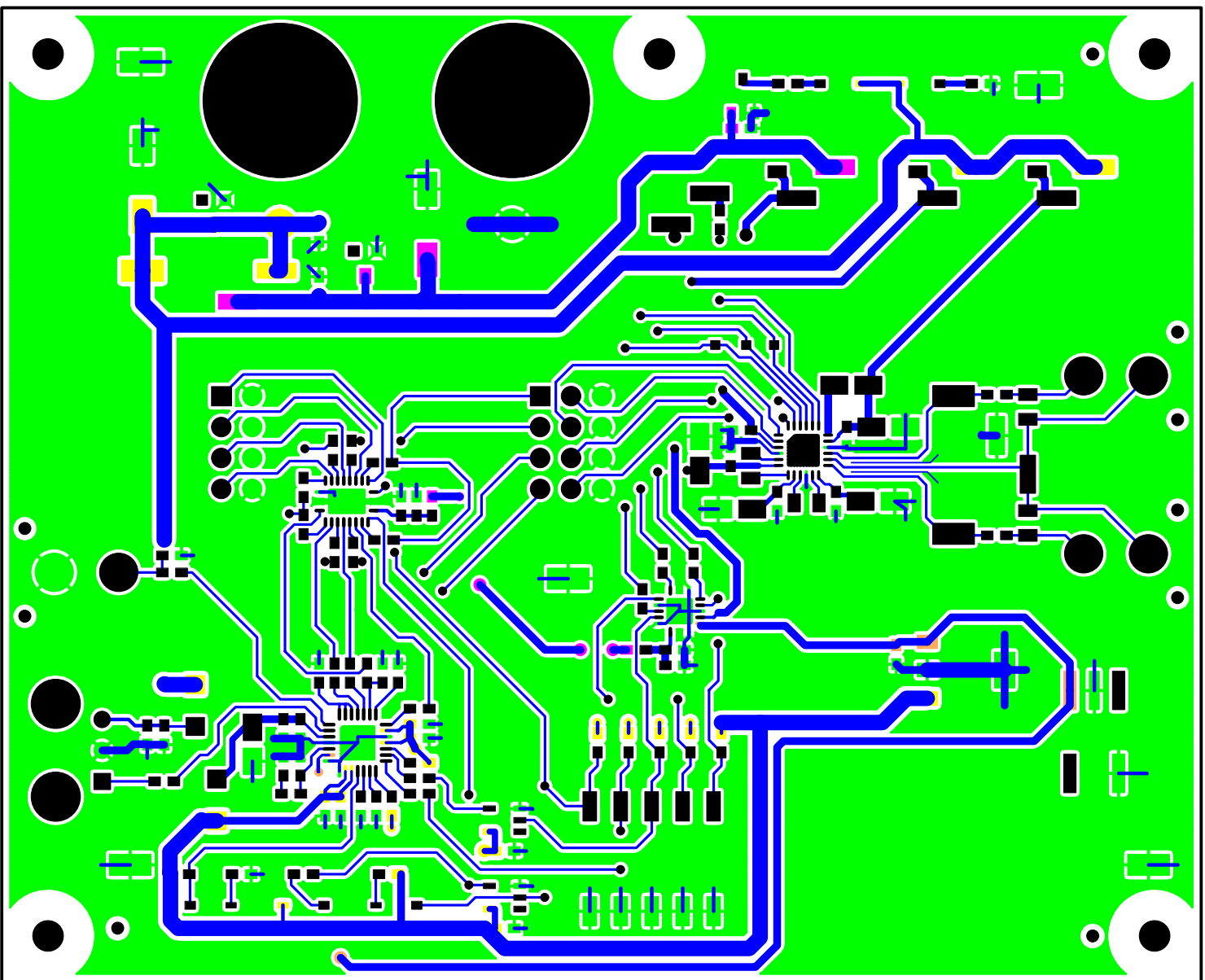
Figure 35. Top Side
