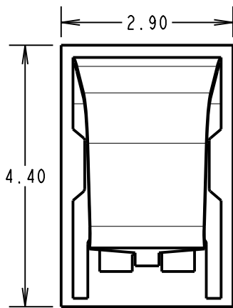
RECOMMENDED PAD LAYOUT
