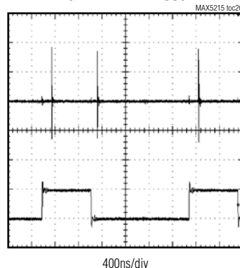
DIGITAL FEEDTHROUGH
