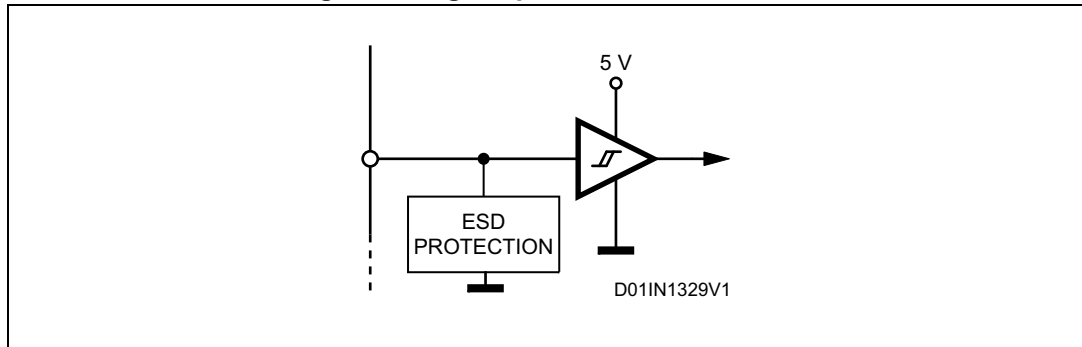
Figure 7. EN_A and EN_B pins open collector driving
