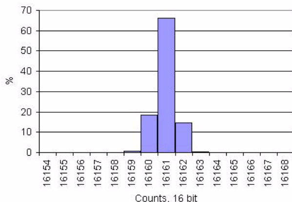
Figure 11-29. Delta-sigma ADC Noise Histogram, 1000 Samples, 16-bit, 48 ksp, Ext Ref, V_{IN} = V_{REF}/2 , Range = \pm 1.024 V
