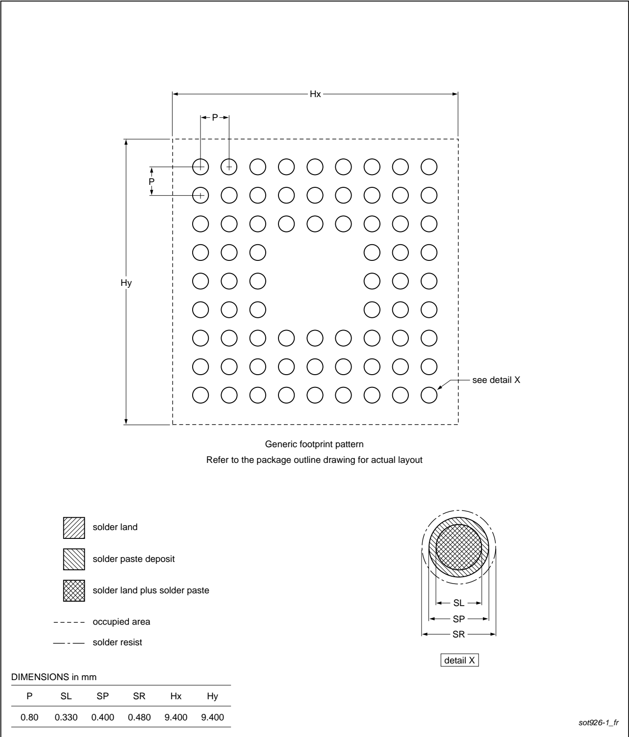
Fig 44. Reflow soldering of the TFBGA100 package
