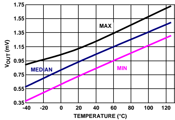
FIGURE 34. V_{OUT} LOW vs TEMPERATURE, V_+ = 5V , V_- = 0V , V_{CM} = 2.5V , R_L = 100k
