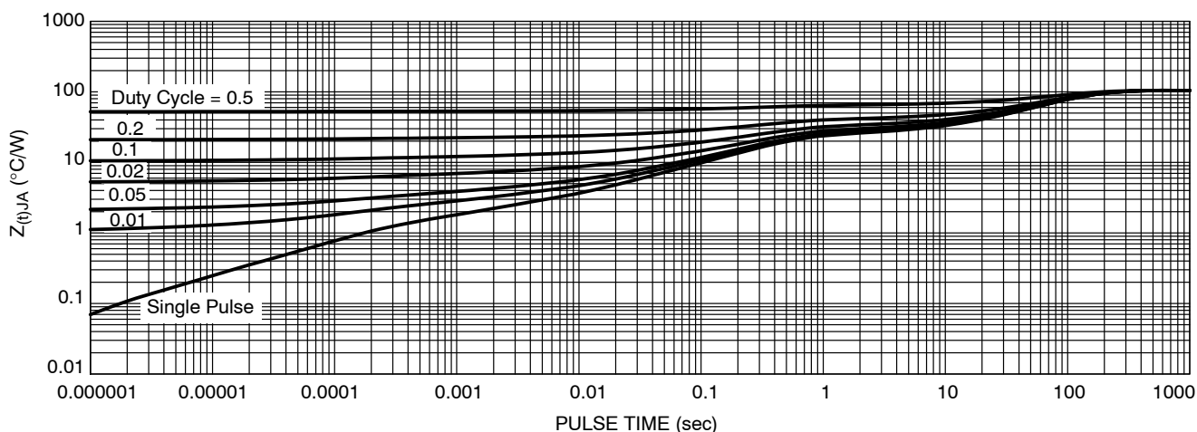
Figure 42. Junction-to-Ambient Transient Thermal Impedance (minimum pad size)
