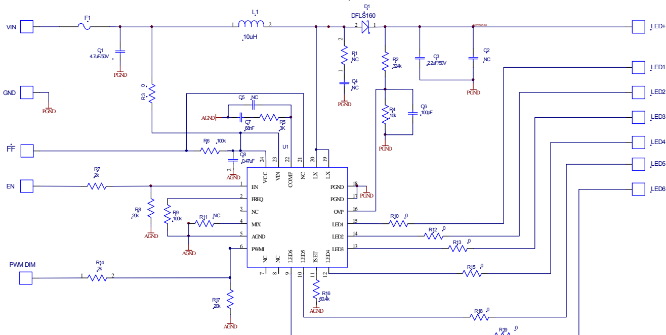
Figure 2: Vin<5.5V,6string,20mA/string application
