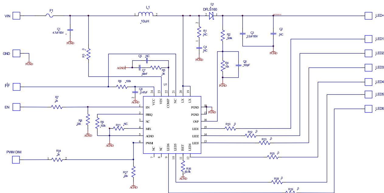
Figure 1: Vin>5.5V,6string,20mA/string application
