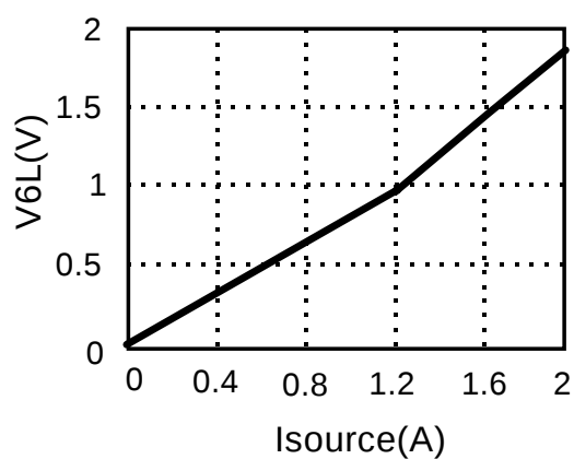
Figure 4. I_{source} - V_{6L}
