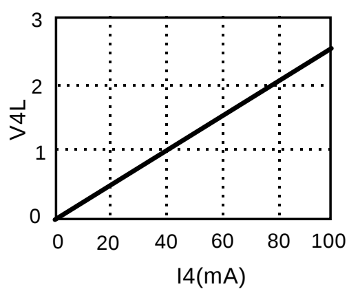
Figure 2. I_4 - V_{4L}
