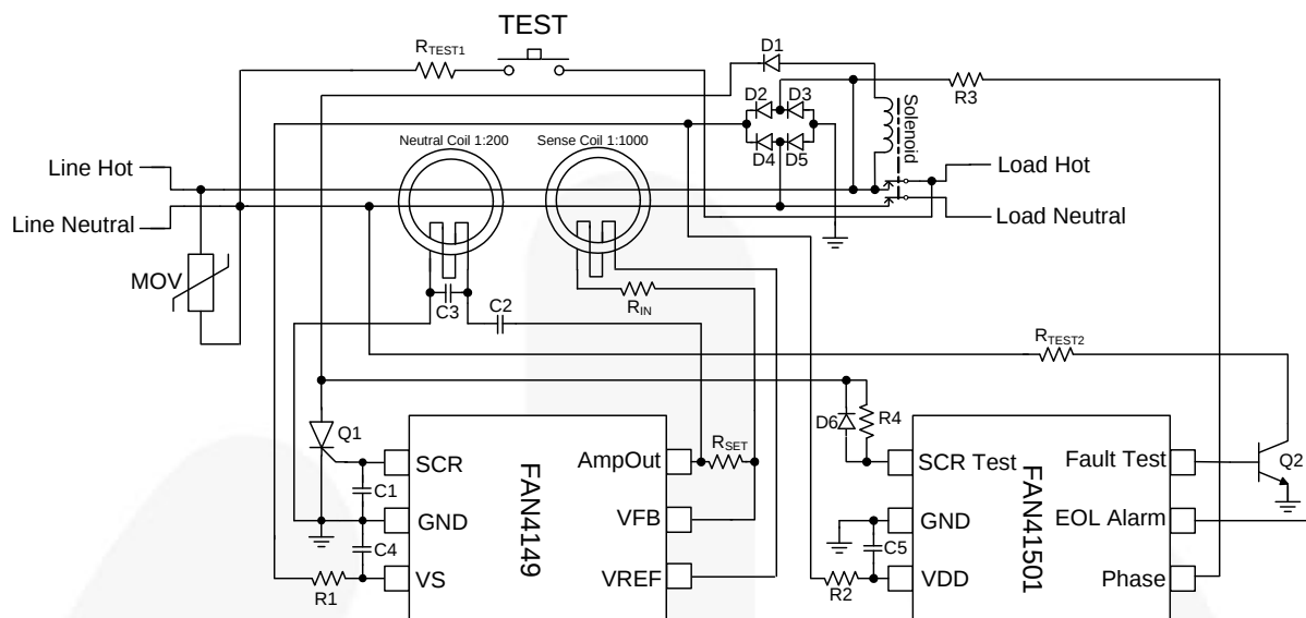
Figure 1. Typical Application (1,2)
