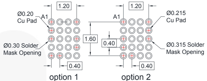
option 1 option 2 RECOMMENDED LAND PATTERN (NSMD TYPE)
