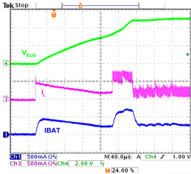
Figure 31. Startup, 3.6\text{ V}_{BAT} , 44\ \Omega Load, Additional 10\ \mu\text{F} , X5R Across V_{BUS}
