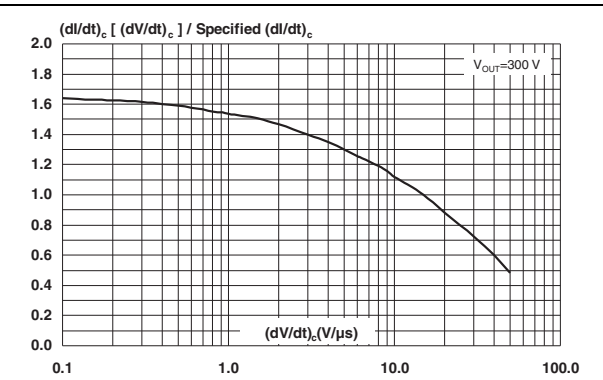
Figure 9. Relative variation of critical rate of decrease of main current versus reappplied dV/dt (typical values)
