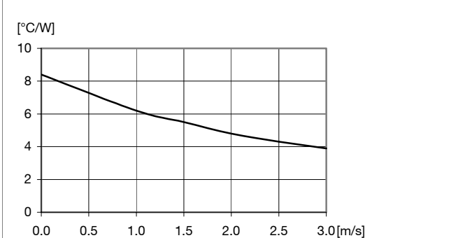
Thermal resistance vs. airspeed measured at the converter. Tested in wind tunnel with airflow and test conditions as per the Thermal consideration section. V_i = 53\text{ V} .
