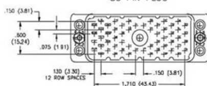
56 PIN PLUG
