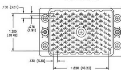
120 PIN PLUG
