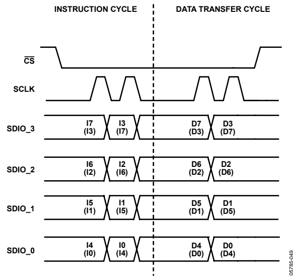
Figure 52. 4-Bit Mode Write Timing—Clock Stall Low
