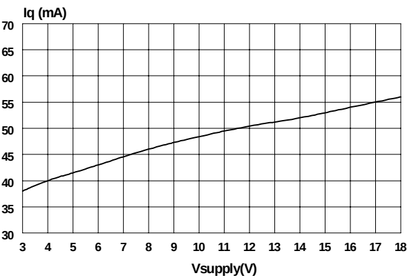
Figure 12: Quiescent Current vs. Supply Voltage
