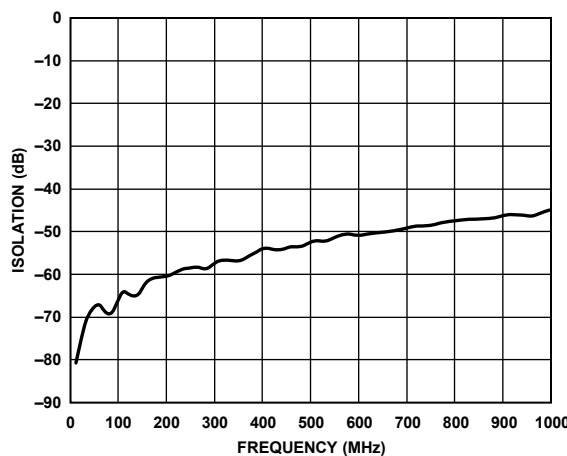
Figure 9. Isolation vs. Frequency ( A_V = 10\text{ dB} )
