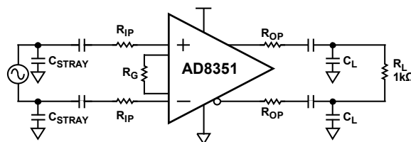
Figure 43. Input and Output Parasitic Suppression Resistors, R_{IP} and R_{OP} , Used to Suppress Capacitive Loading Effects
