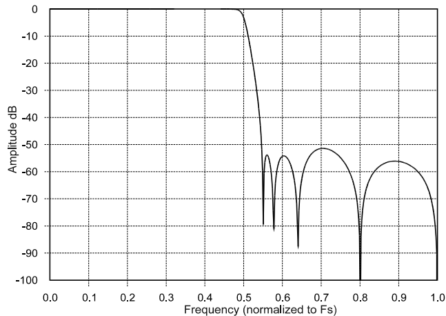
Figure 15. Stopband Rejection
