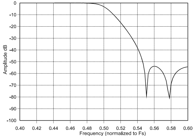
Figure 16. Transition Band
