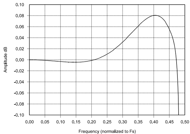
Figure 18. Passband Ripple
