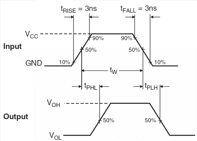
Figure 6. AC Waveforms
