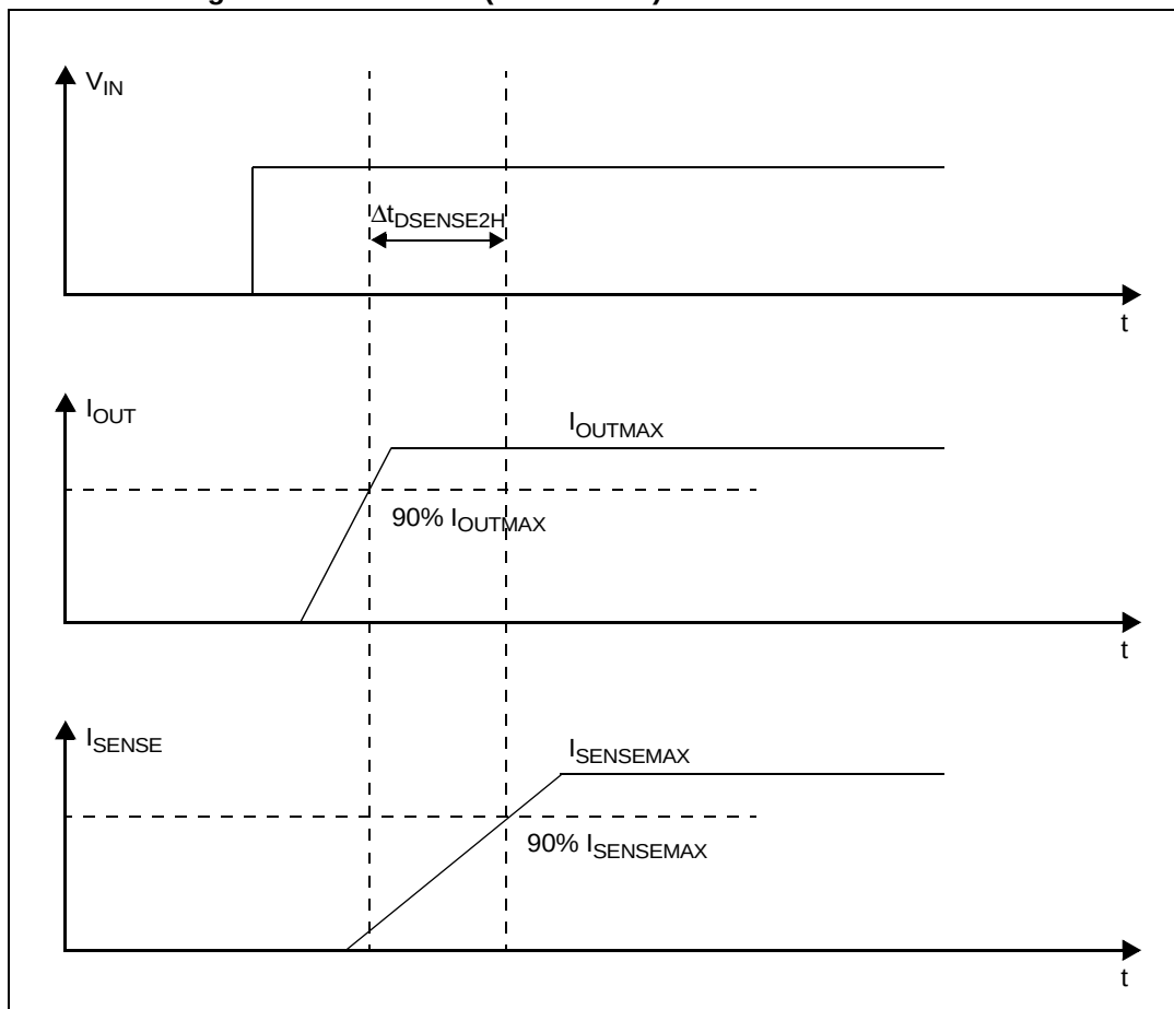
Figure 7. Switching characteristics
