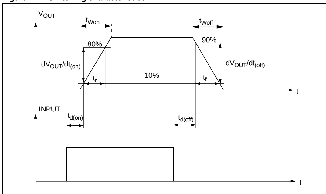
Figure 7. Switching characteristics
