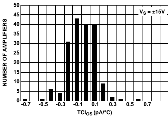
FIGURE 19. TC 1os- vs NUMBER OF AMPLIFIERS, V S = ±15V
