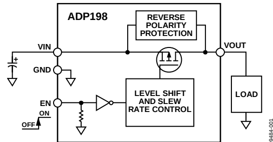
Figure 1. WLCSP
