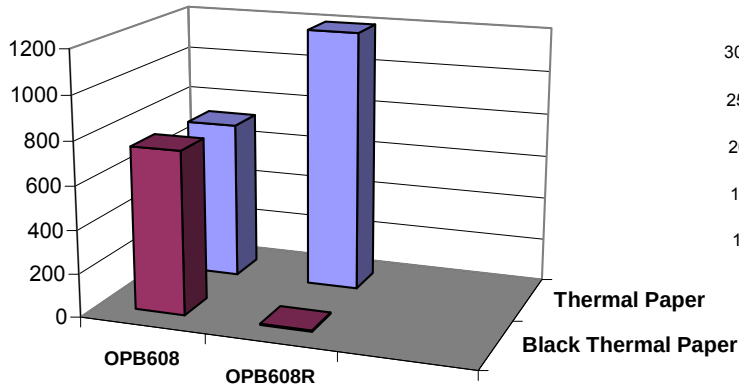
Reflective Response
