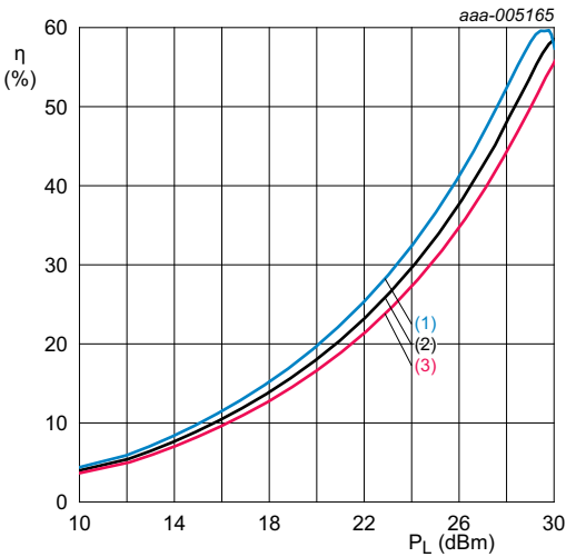
T_{amb} = 25\text{ }^{\circ}\text{C} ; I_{CC(tot)} = 70\text{ mA} ; matched for ISM-434. (1) V_{SUP} = 3.3\text{ V} (2) V_{SUP} = 3.6\text{ V} (3) V_{SUP} = 3.9\text{ V}
