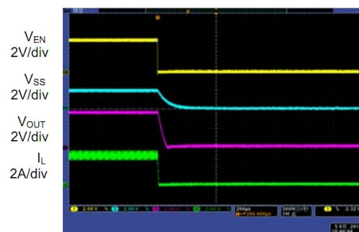
Fig. 13: Enable turn off CC mode, V_{IN}=12V , V_{OUT}=V_{EN}=3.3 , I_{OUT}=3A
