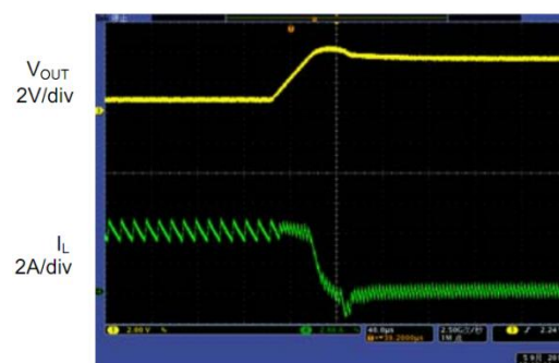
Fig. 15: Short-circuit recovery
