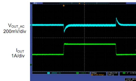
Fig. 11: Load transient ( I_{OUT}=1.5A to 3A )
