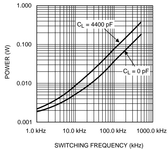
Figure 20. Diode Power Dissipation V_{IN} = 40V
