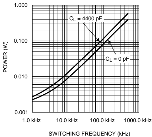
Figure 19. Diode Power Dissipation V_{IN} = 80V
