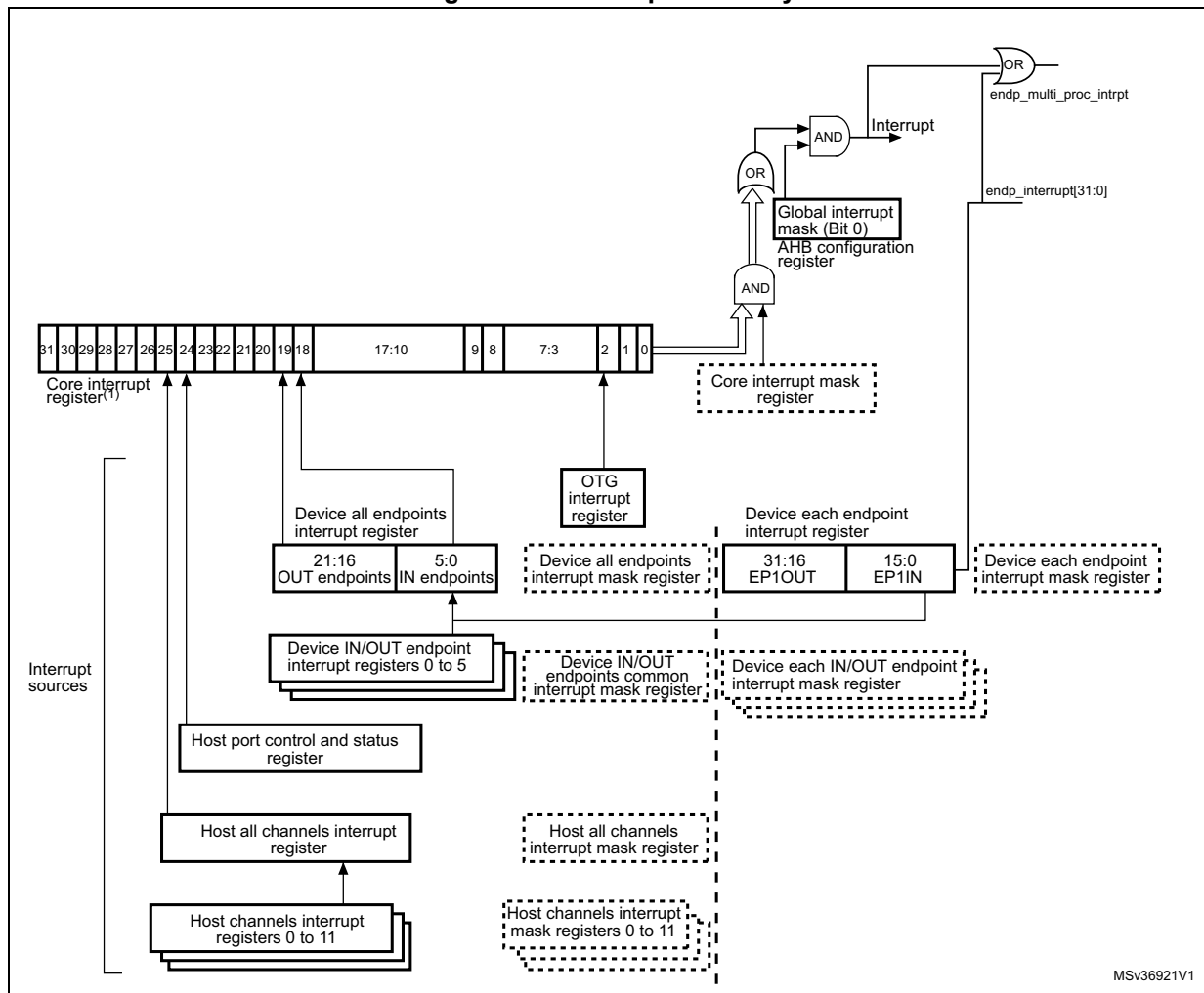
Figure 449. Interrupt hierarchy
