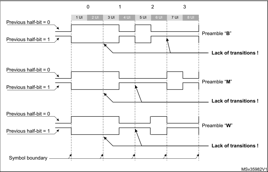
Figure 397.S/PDIF Preambles
