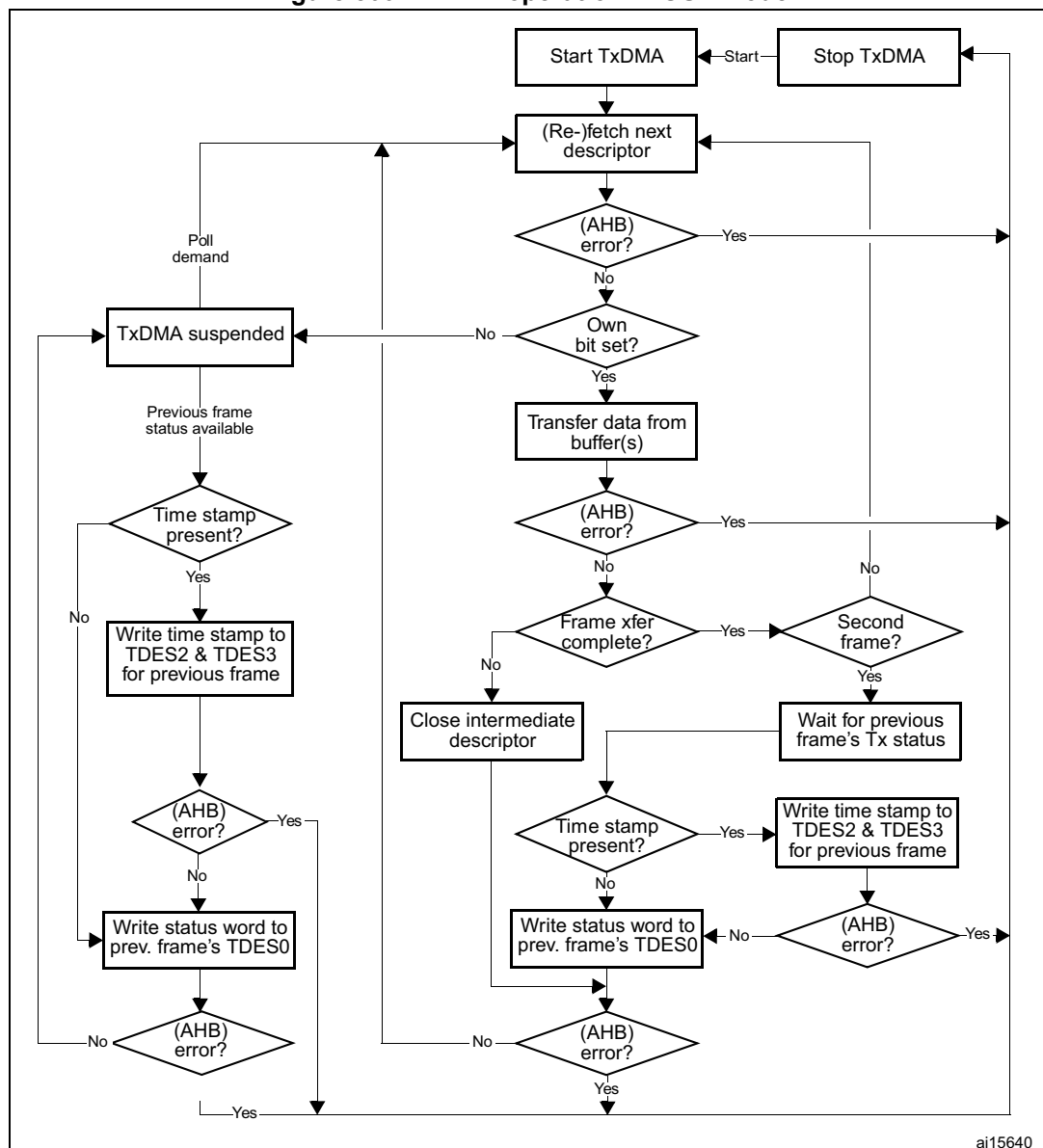
Figure 500. TxDMA operation in OSF mode
