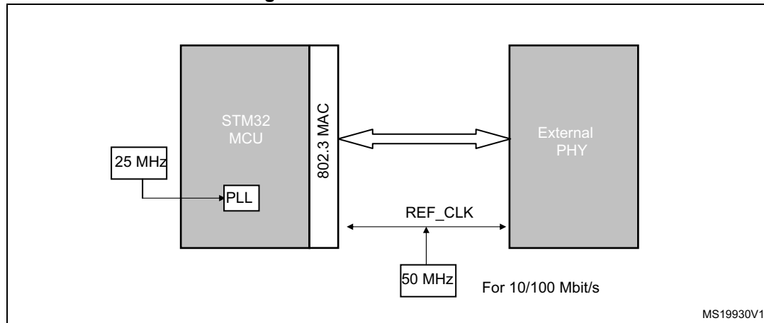
Figure 479. RMII clock sources-
