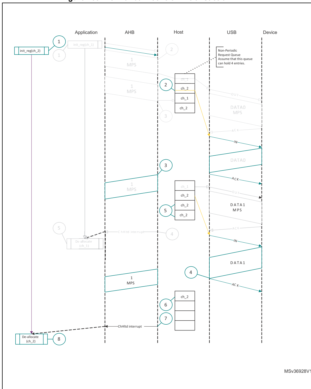
Figure 459. Normal bulk/control IN transaction - DMA
