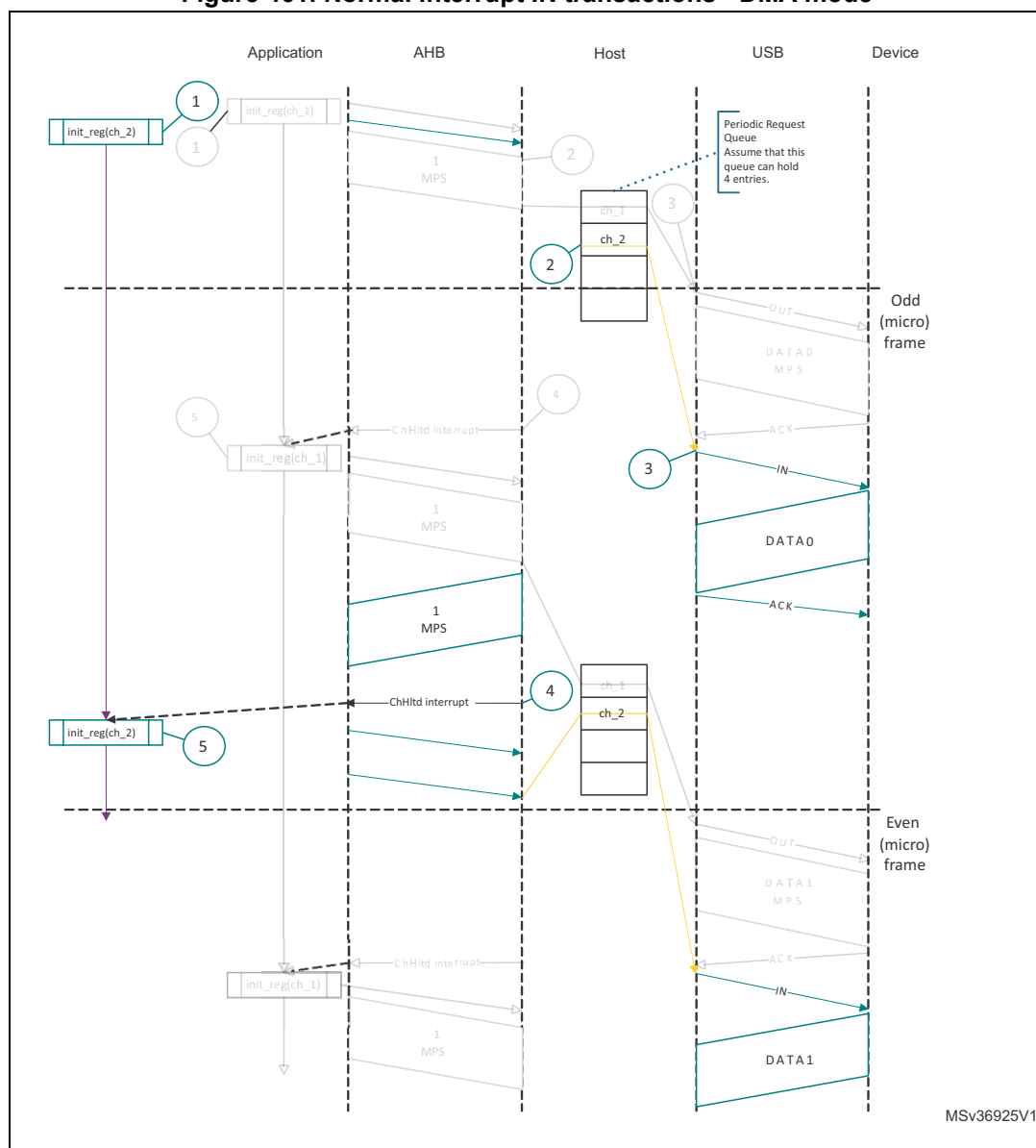
Figure 461. Normal interrupt IN transactions - DMA mode
