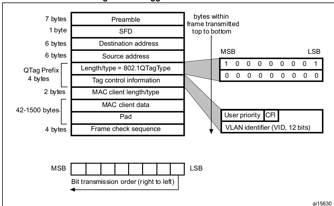
Figure 483. Tagged MAC frame format
