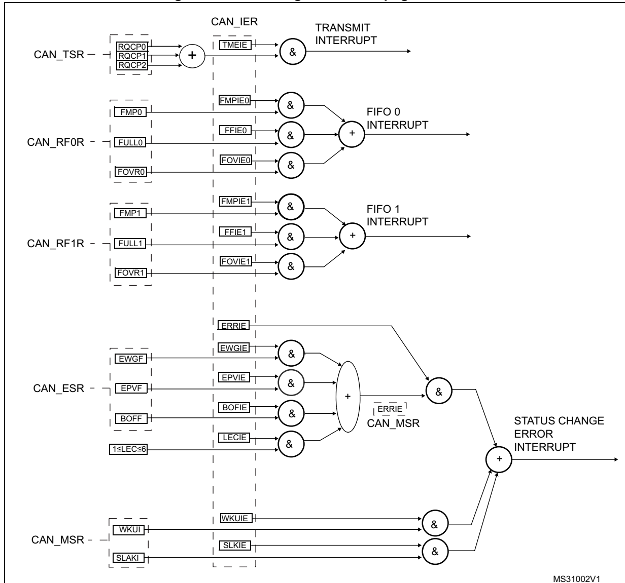
Figure 438. Event flags and interrupt generation
