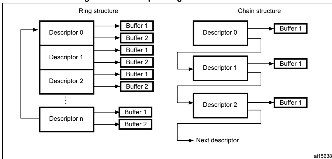
Figure 498. Descriptor ring and chain structure
