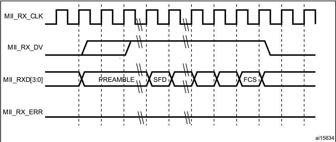
Figure 489. Reception with no error
