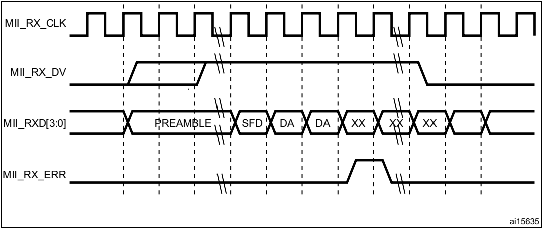
Figure 490. Reception with errors
