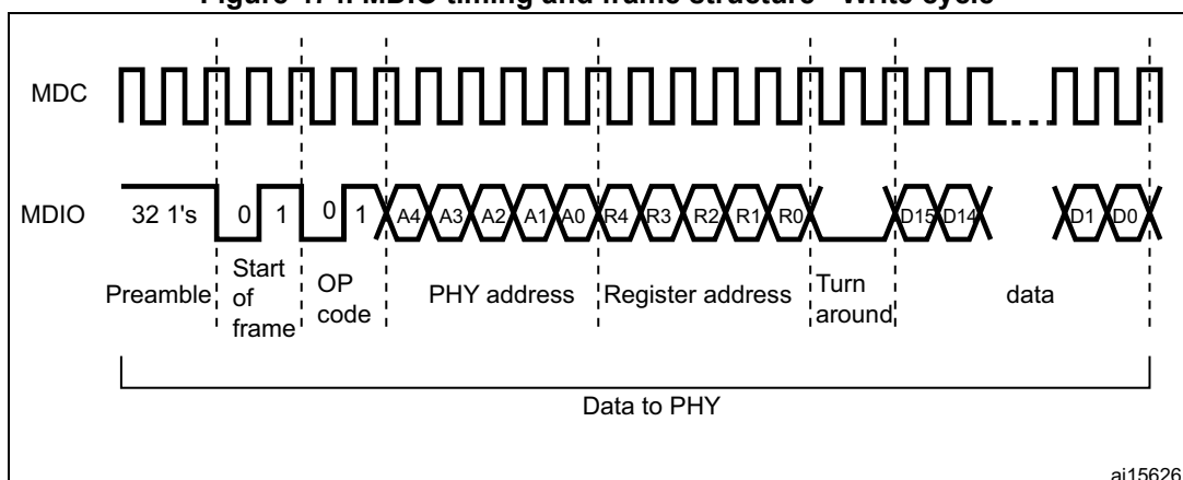
Figure 474. MDIO timing and frame structure - Write cycle
