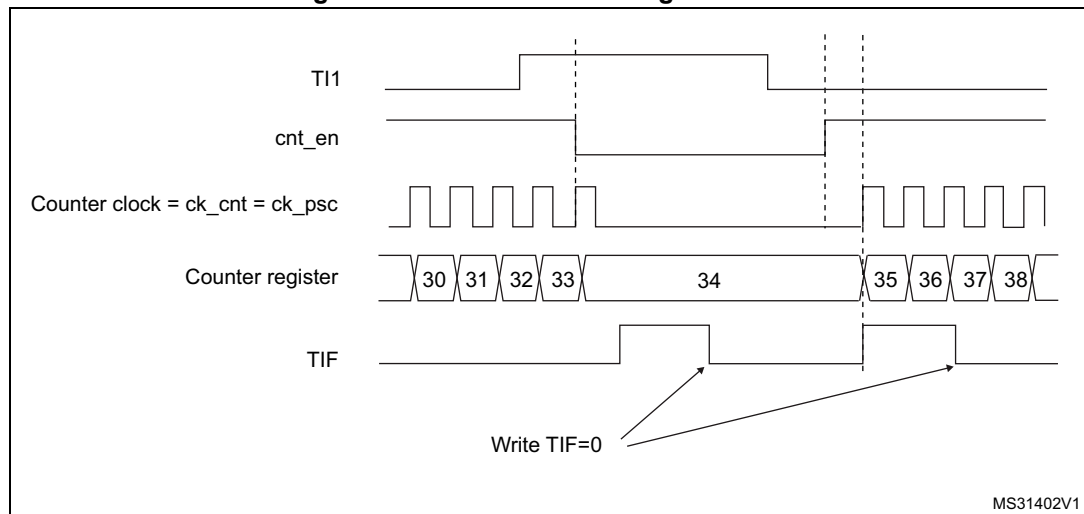
Figure 262. Control circuit in gated mode
