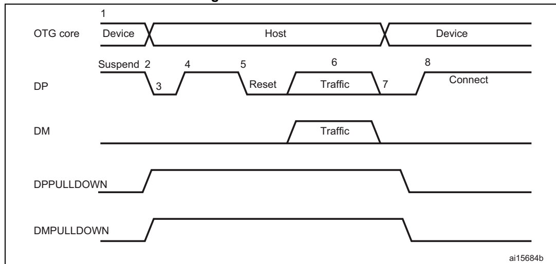
Figure 471. B-device HNP
