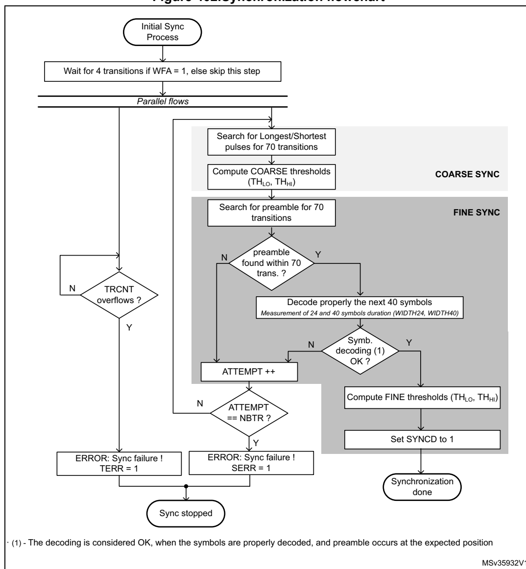
Figure 402. Synchronization flowchart
