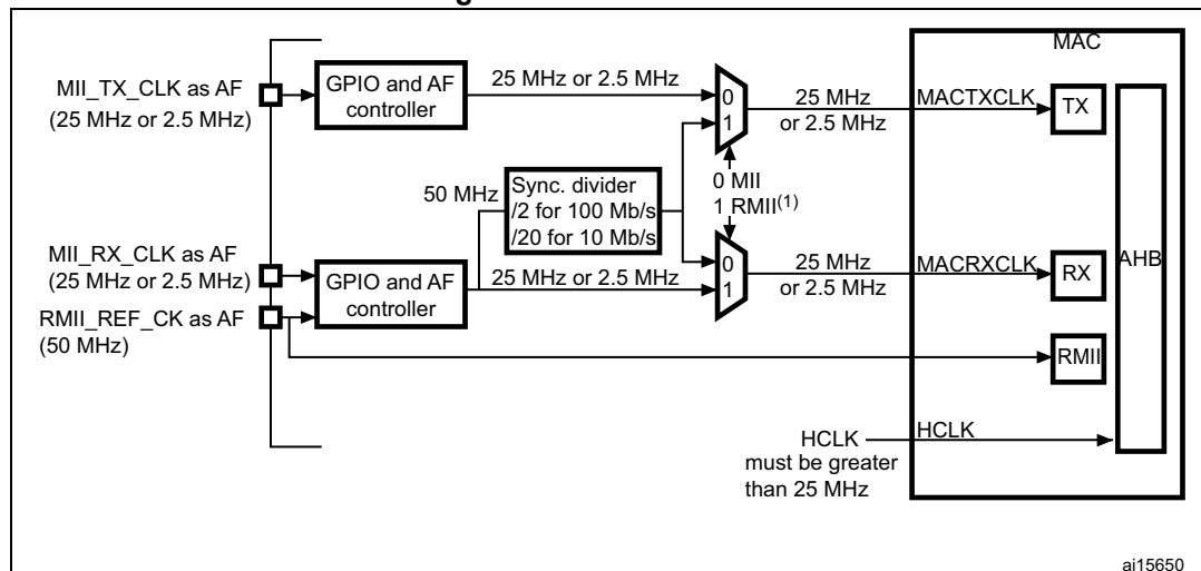
Figure 480. Clock scheme
