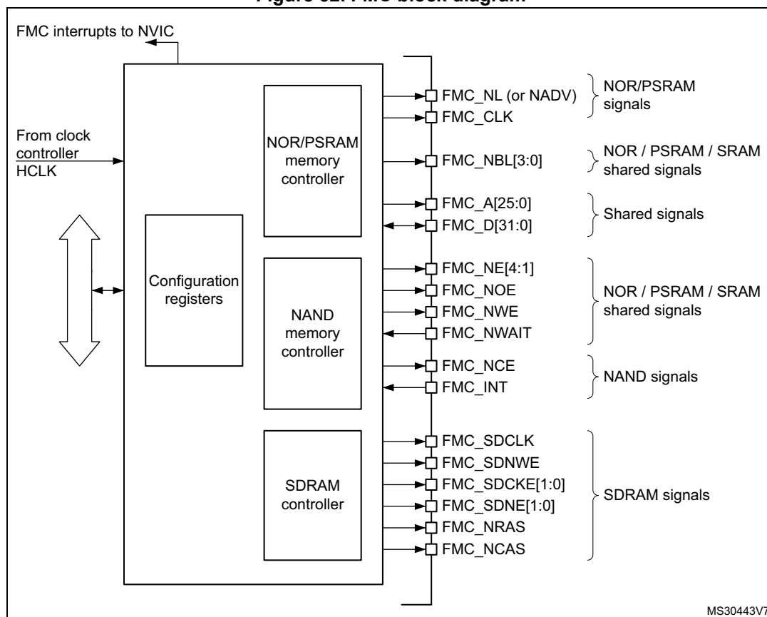
Figure 32. FMC block diagram
