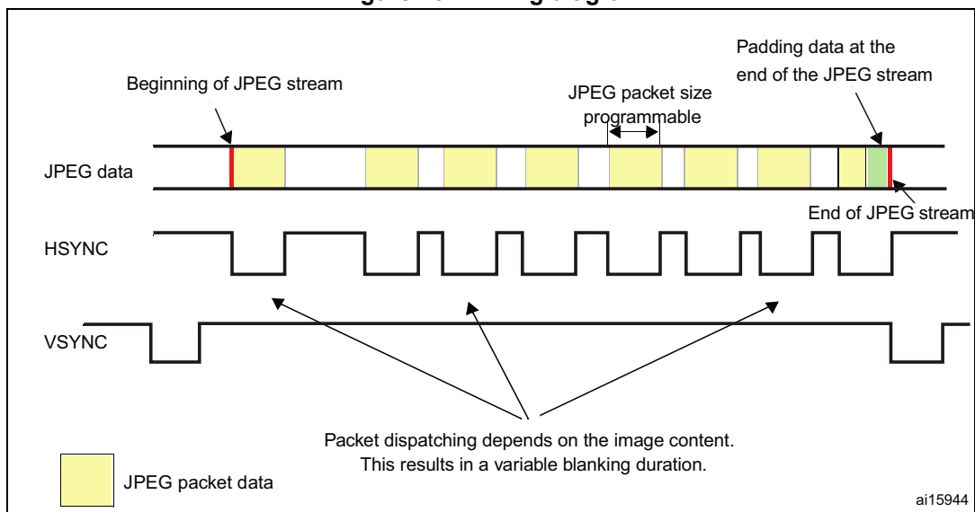
Figure 104. Timing diagram
