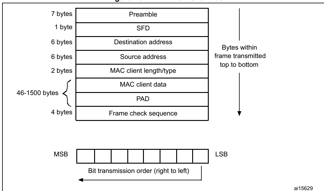
Figure 482. MAC frame format
