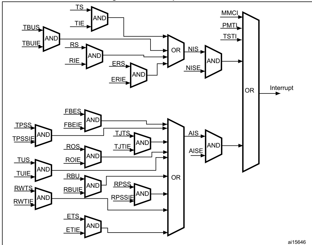
Figure 506. Interrupt scheme
