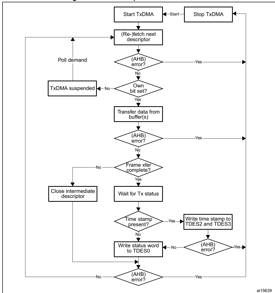
Figure 499. TxDMA operation in default mode
