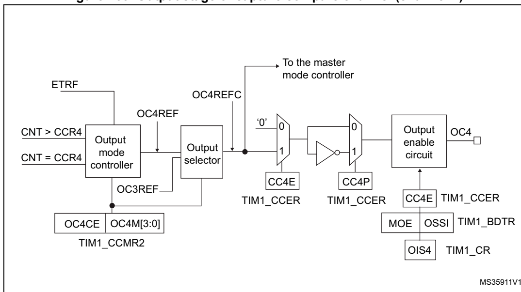
Figure 163. Output stage of capture/compare channel (channel 4)
