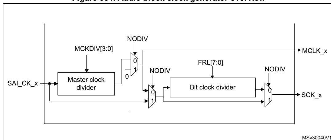
Figure 384. Audio block clock generator overview
