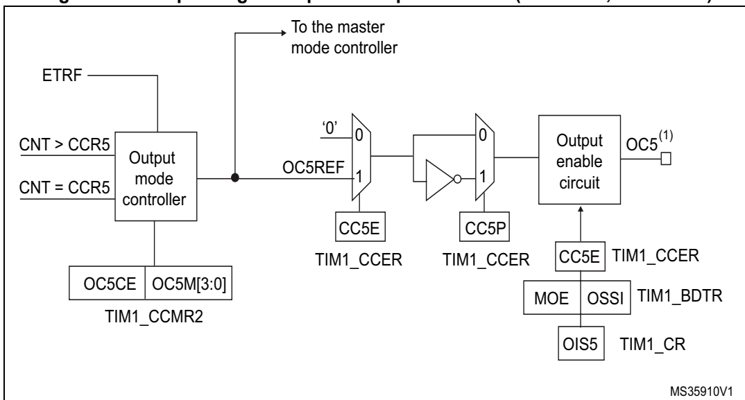
Figure 164. Output stage of capture/compare channel (channel 5, idem ch. 6)
