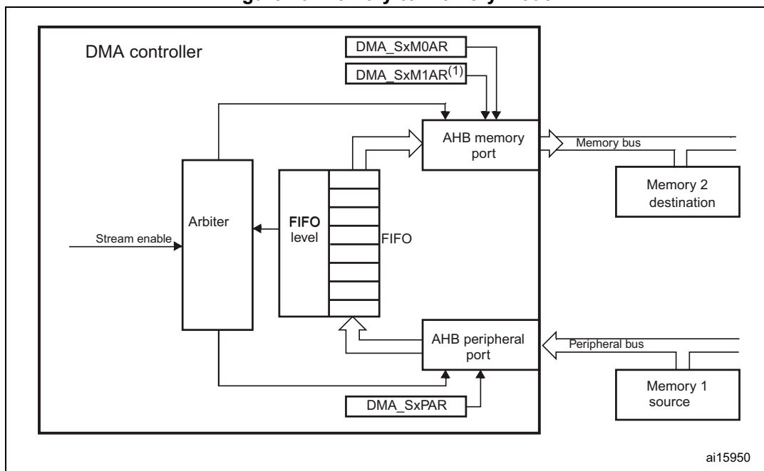
Figure 26. Memory-to-memory mode
