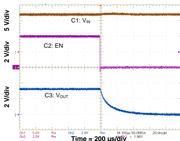
Figure 20. Shutdown Relative to EN
