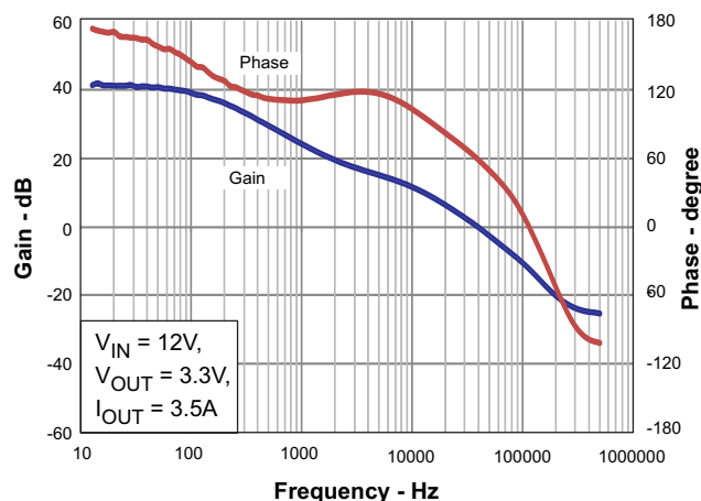
Figure 9. Loop Response
