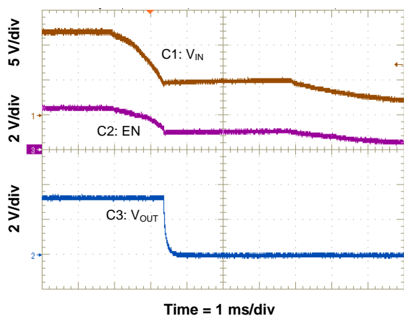
Figure 19. Shutdown Relative to V_{IN}
