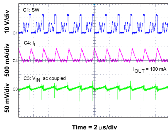
Figure 15. Input Voltage Ripple DCM
