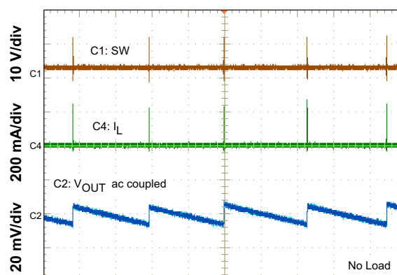
Figure 13. Output Voltage Ripple Eco-mode
