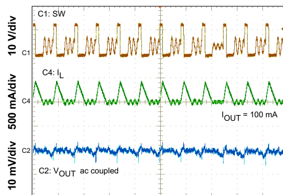
Figure 12. Output Voltage Ripple DCM
