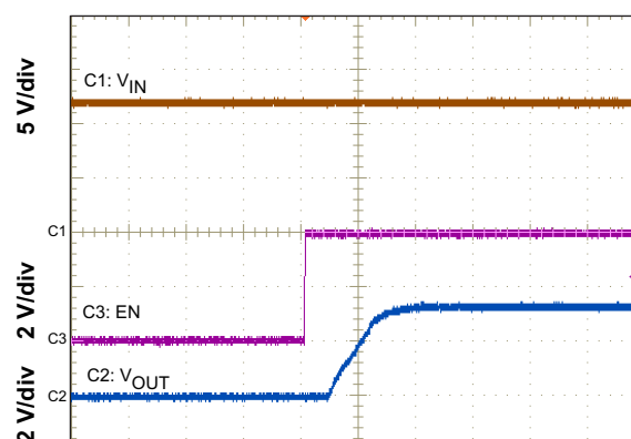
Time = 2 ms/div Figure 17. Start Up Relative to EN
