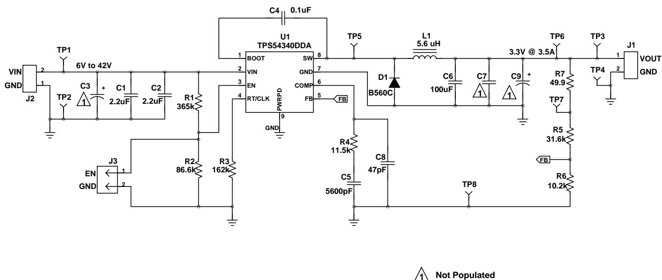
Figure 28. TPS54340EVM-182 Schematic
