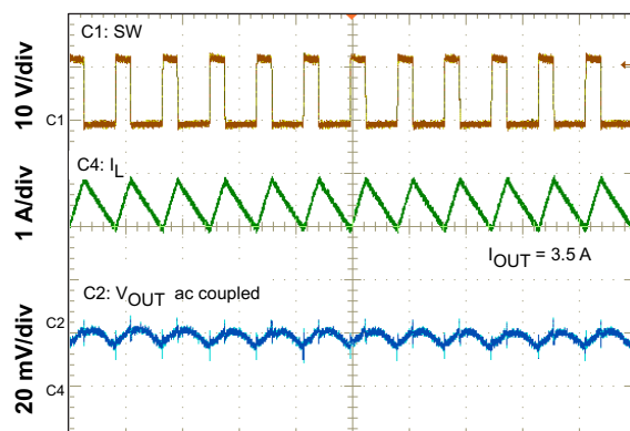
Figure 11. Output Voltage Ripple CCM
