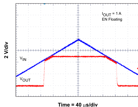
Figure 22. Low Dropout Start Up and Shutdown
