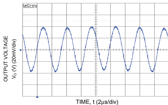
Figure 9. Typical Output Ripple and Noise ( V_{IN} = 12\text{ V dc} , V_O = 3.3\text{ Vdc} , I_O = 16\text{ A} ).
