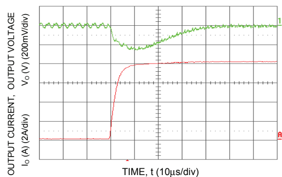
Figure 12. Transient Response to Dynamic Load Change from 50% to 100% of full load ( V_O = 3.3\text{ Vdc} , C_{ext} = 2 \times 150\text{ }\mu\text{F} Polymer Capacitors).
