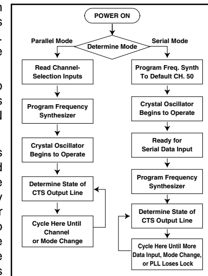
Figure 10: Start-up Sequence
