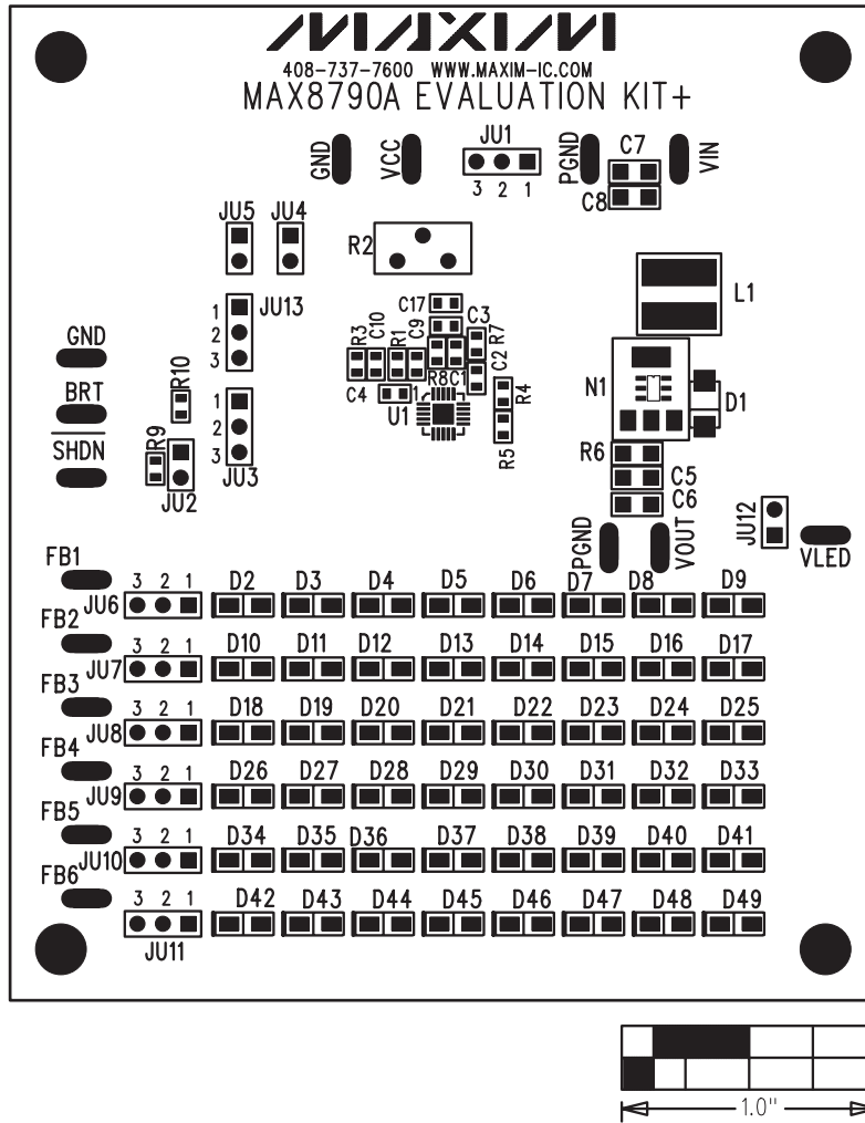
Figure 2. MAX8790A EV Kit Component Placement Guide—Component Side
