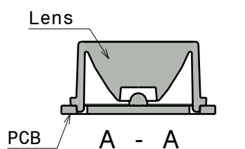
PCB suggestion
