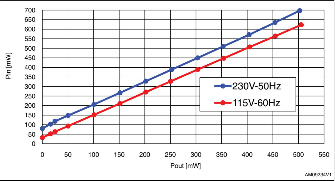
Figure 1. Standby consumption
