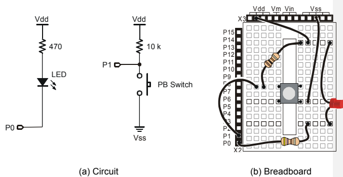
Program Listing 2.3 - Flash LED with Pushbutton
