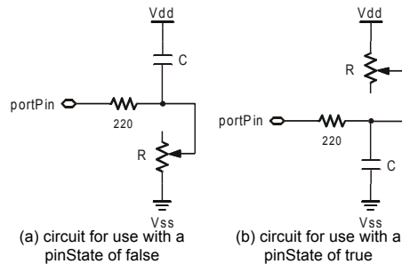
Figure 9.6 RCTime circuits for recommended
