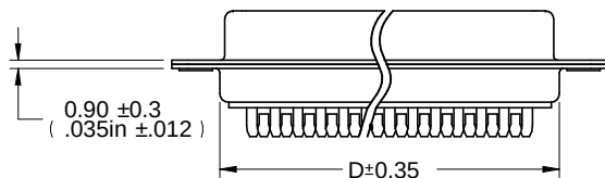
DIM OUTLINE
