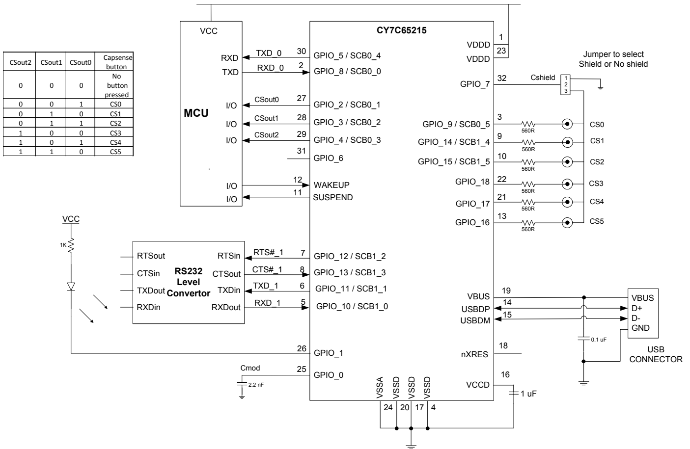
Figure 10. CapSense Schematic
