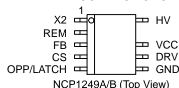
NCP1249A/B (Top View)
