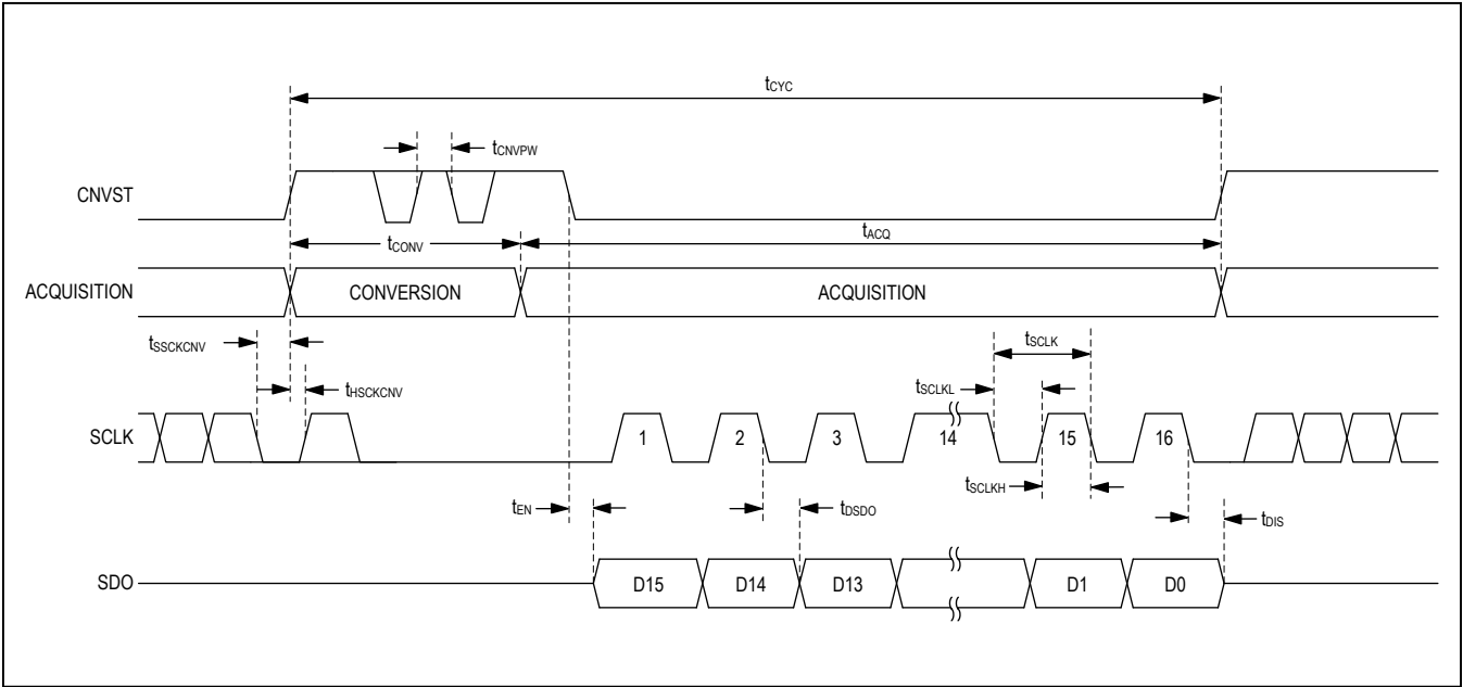
Figure 6. \overline{CS} Mode 3-Wire, No-Busy Indicator Serial Interface Timing ( \overline{SDI} High)
