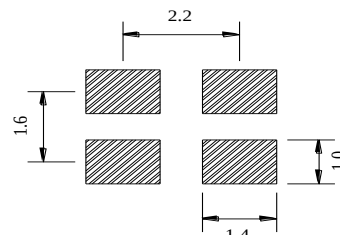
<SUGGESTED LAYOUT>
