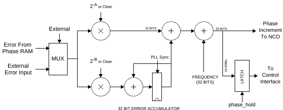
Figure 5. PLL CIRCUIT
