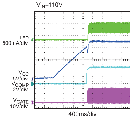
V_{IN} Startup
