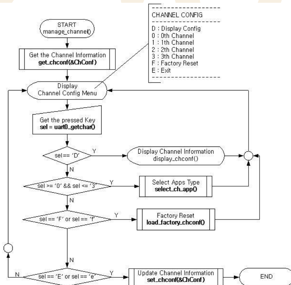
<Fig 3.7: manage_channel()>
