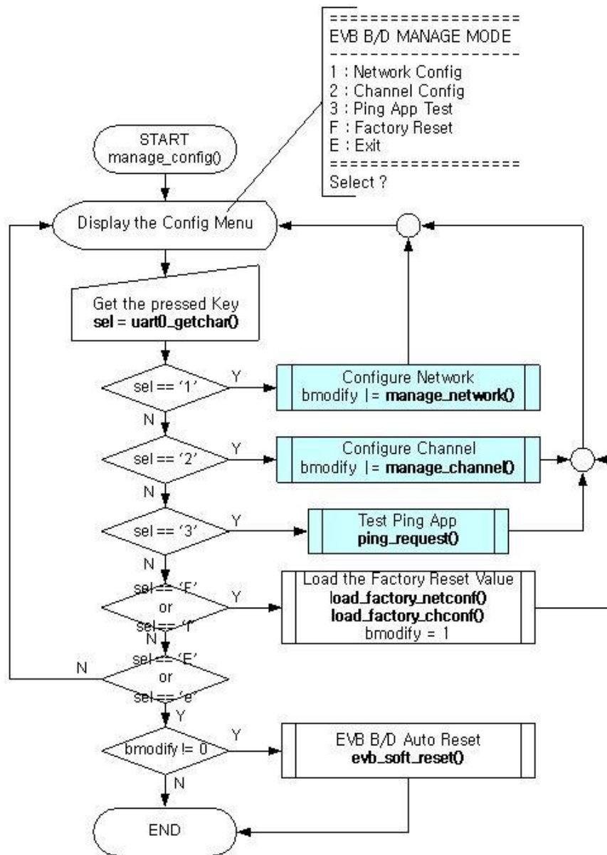
<Fig 3.5: manage_config()>
