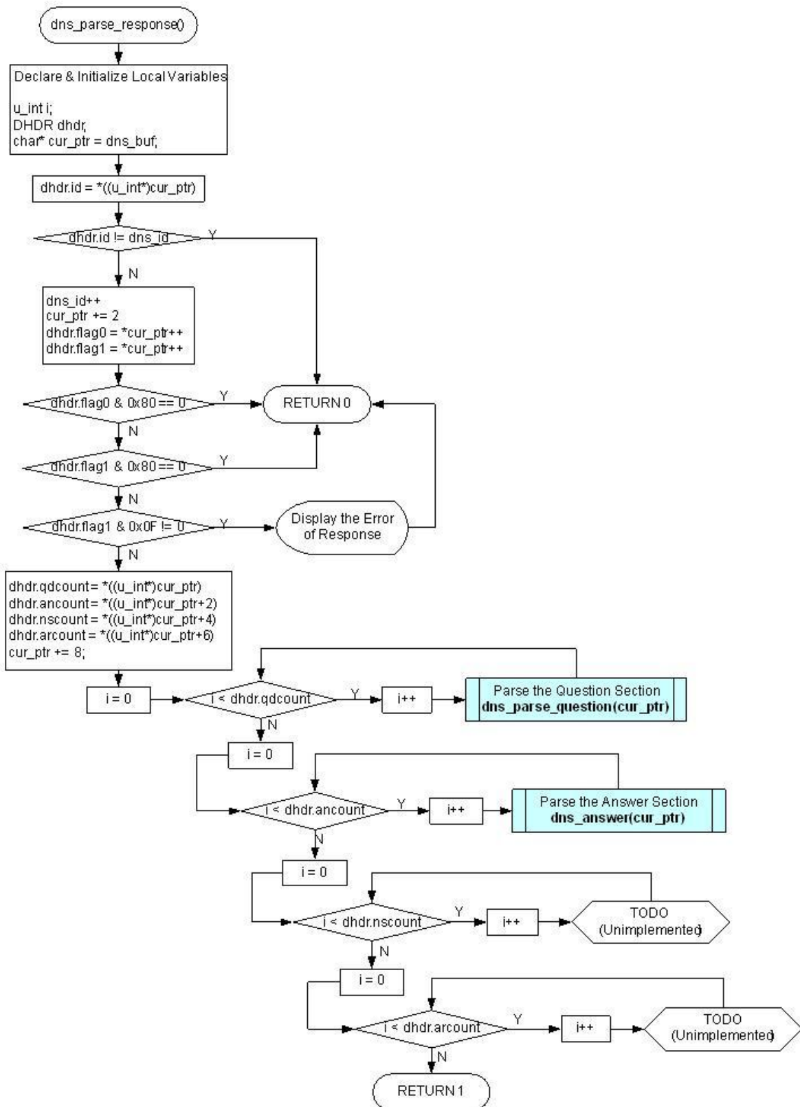
<Fig 3.42: dns_parse_response()>
