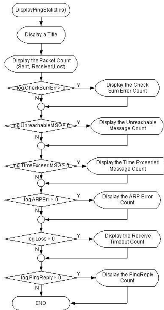
<Fig 3.12: DisplayPingStatistics()>
