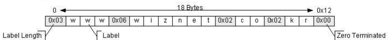
<Fig 3.41: Example of QNAME Field transformation of Question Section >
