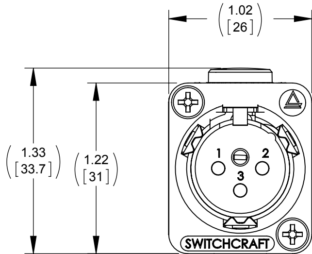
MALE XLR MONO OUTPUT
