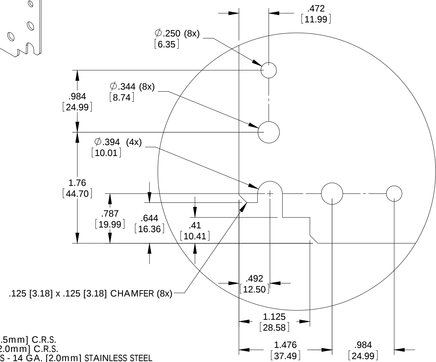
DETAIL A SCALE 2 : 1.75
