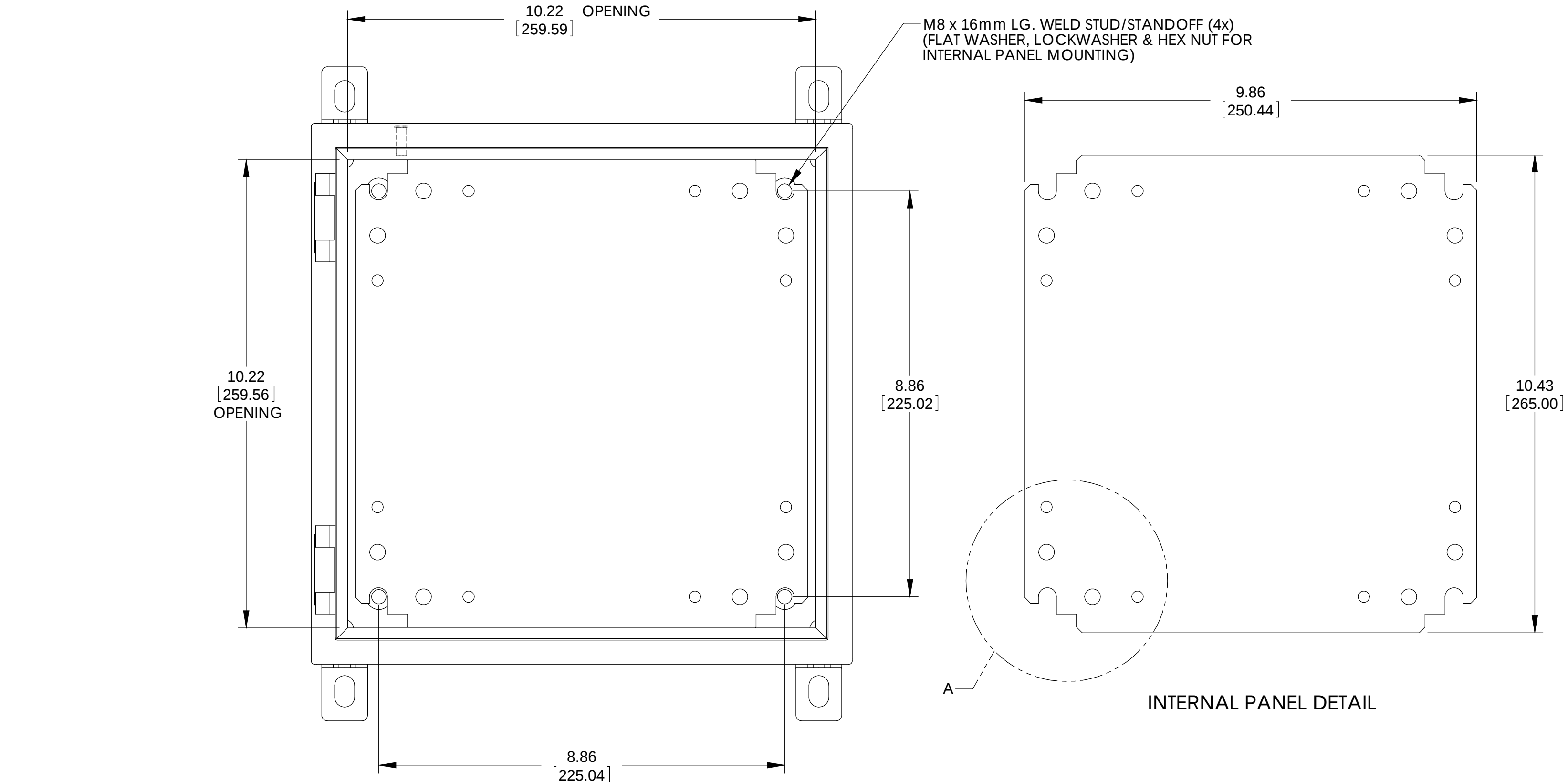
FRONT VIEW (LESS COVER)
